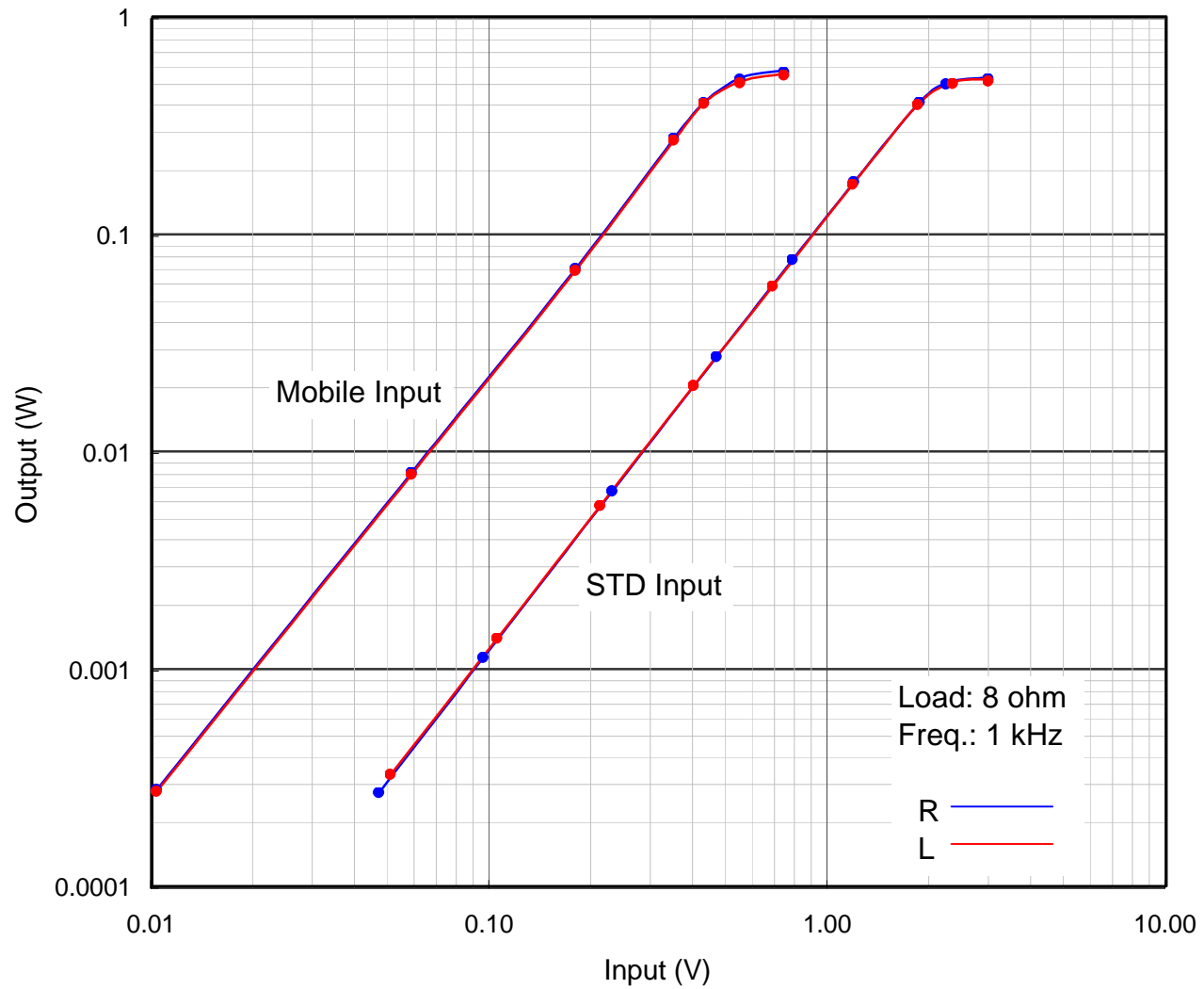
E180F Single Ended Single Stage Amplifier - Input/Output Plot
