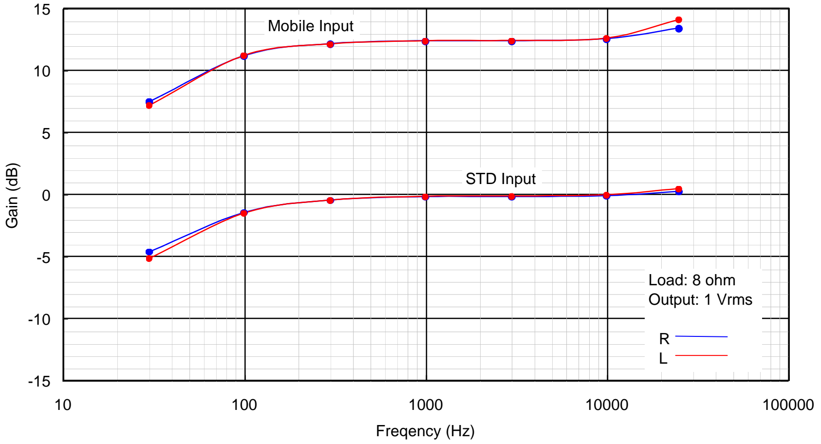
E180F Single Ended Single Stage Amplifier - Freq. Response Plot
